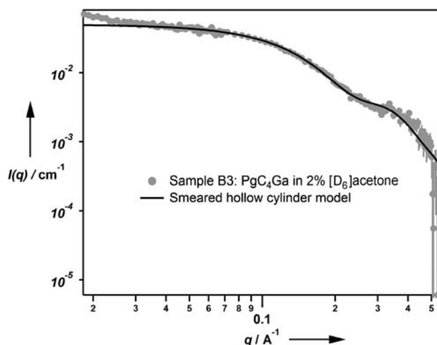
Figure 2. SANS data for the gallium-seamed C-butylpyrogallol[4]arene nanocapsule. A resolution-smeared hollow cylinder model is fitted to the SANS data (see text). Error bars on the SANS data represent one standard deviation.
